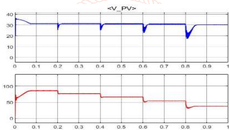
Fig 7 (a): Voltage vs Time in (S) in correspondence with P&O Method.
