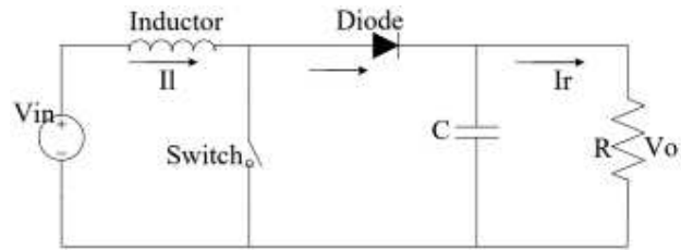
Fig. 2: Circuit Diagram of Boost Converter
