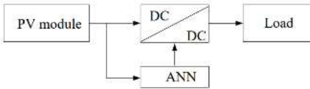
Fig. 4: MPPT System with ANN Controller
