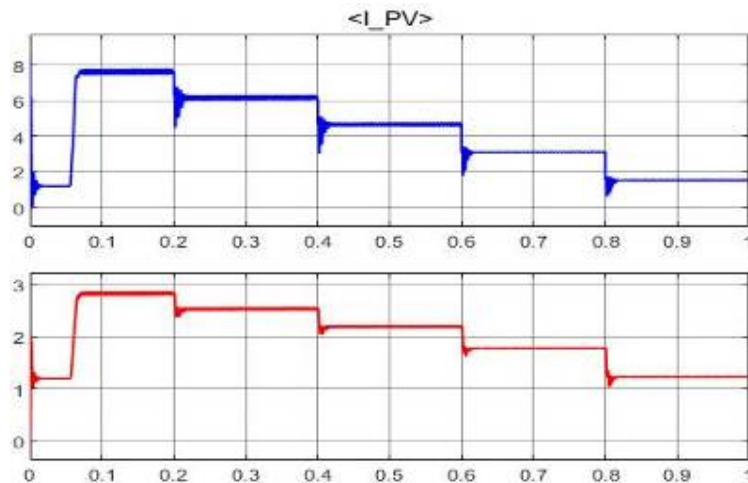
Fig 8 (b): Current vs Time in (S) in correspondence with ANN Method.
