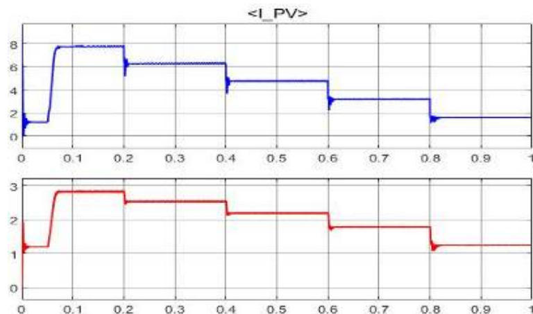
Fig 9 (b): Current vs Time in (S) in correspondence with NN – P&O Method.
