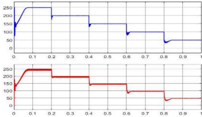
Fig 7 (c): Power vs Time in (S) in correspondence with P&O Method.
