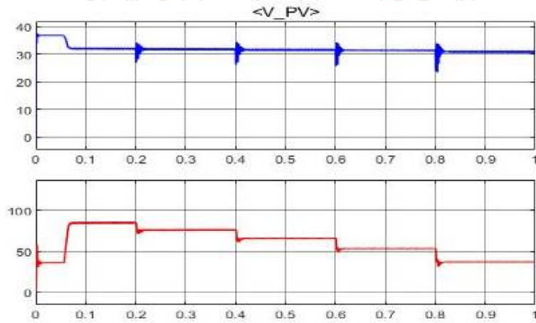
Fig 8 (a): Voltage vs Time in (S) in correspondence with ANN Method.
