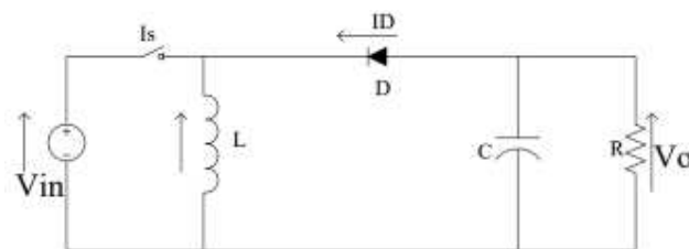
Fig. 3: Circuit Diagram of Boost Converter
