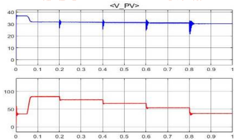
Fig 9 (a): Voltage vs Time in (S) in correspondence with NN – P&O Method.
