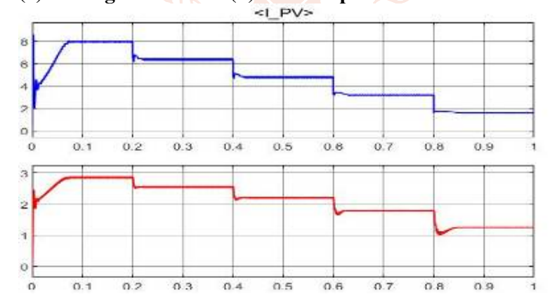
Fig 7 (b): Current vs Time in (S) in correspondence with P&O Method.
