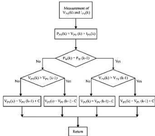
Fig. 5 State-flow Chart of P&O MPPT Technique
