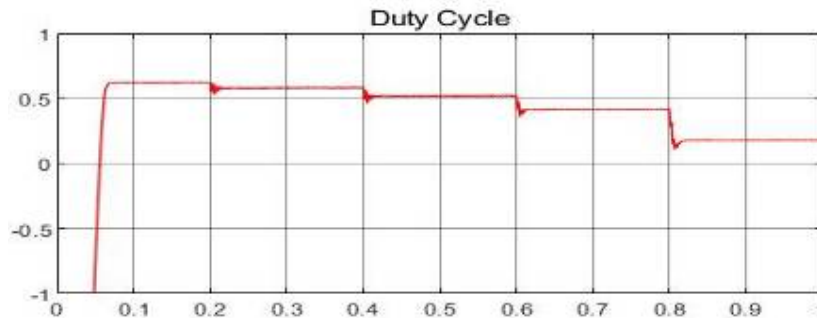
Fig 8 (d): Duty Cycle vs Time in (S) in correspondence with ANN Method.
