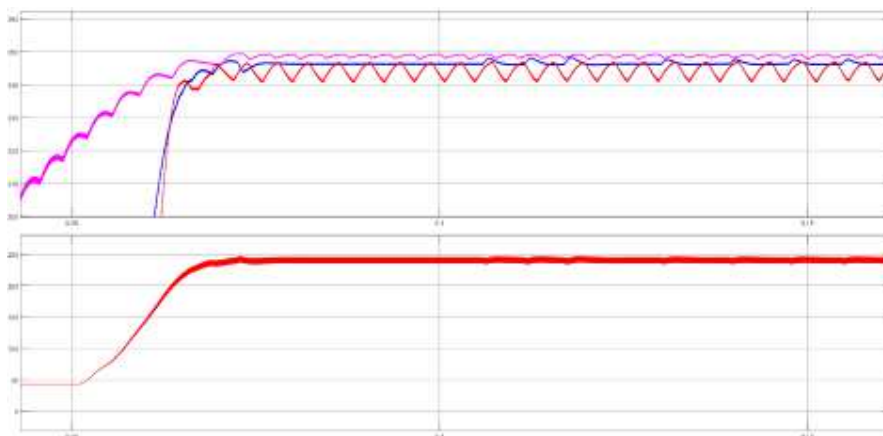
Fig 10 (b): Shows Brief Comparison Between all three techniques
