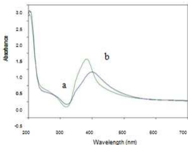
Figure 2. Ag NPs (a) freshly prepared and (b) after 1 week of the synthesis.
