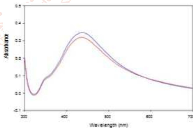
Figure 4. Absorbance spectra of Ag nanoparticles in the presence of vitamin (upper) and vitamin -C low
