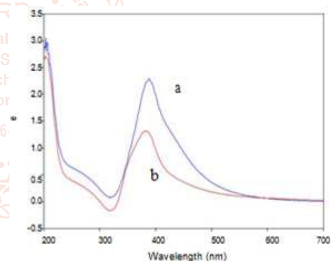
Figure 1. The absorption spectra of Ag NPs using (a) 10 mL of AgNO 3 and (b) 5 mL AgNO 3
