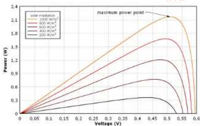
Fig. 2: Relationship between output voltage and power of the PV cell under different irradiation conditions
