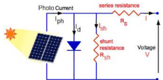
Fig. 1: An equivalent circuit of the PV.
