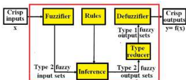
Fig. 3: Type 2 fuzzy inference system structure
