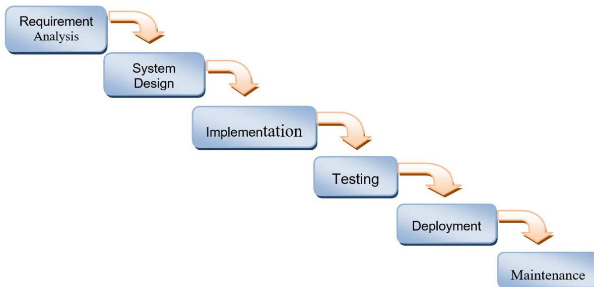
Figure 2 Waterfall Model
