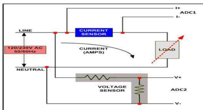
Fig.11 circuit for meter tempering prevention method
