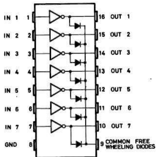
Fig.6 ULN2003 (driver)
