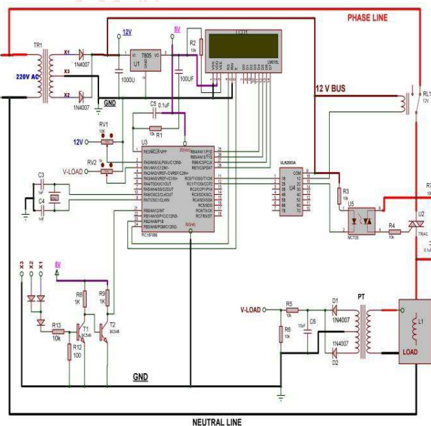
Fig.2 Circuit Diagram of SEM
