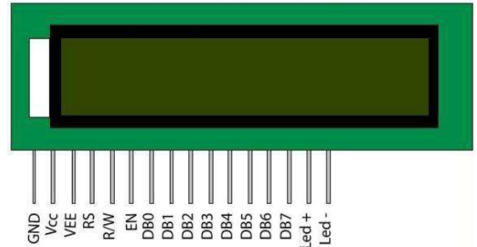
Fig.8 LCD
