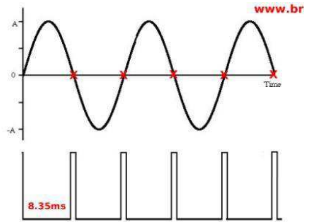
Zero crossing pulse at 0, 180, and 360 degrees.
