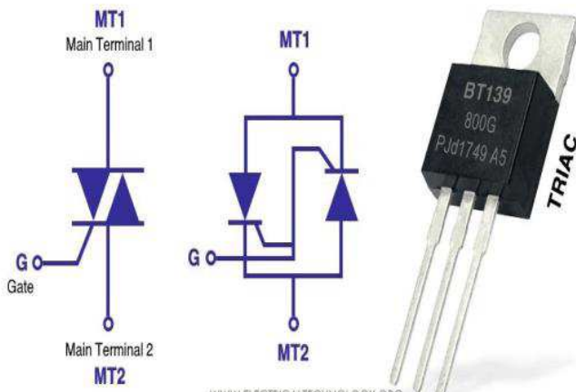
Fig.10 Triac/Transistor
