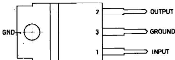
Fig.3.voltage Regulator
