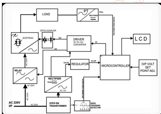
Fig.1 Block Diagram of SEM
