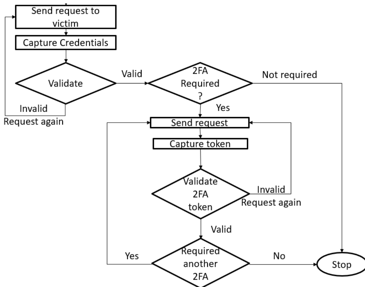
Fig 2 Dataflow diagram
