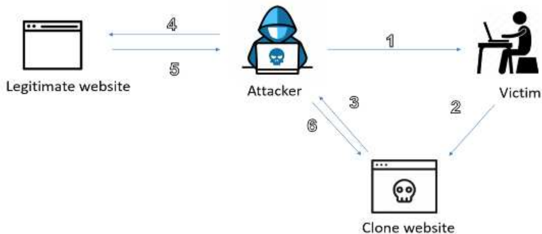
Fig 1 Proposed flow
