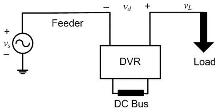
Fig. 1.5: Schematic diagram of DVR.
