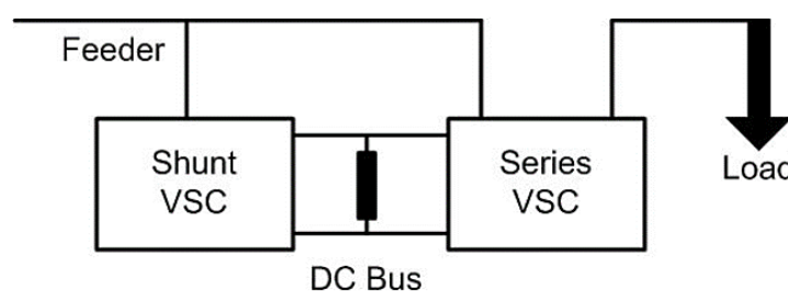
Fig 1.7 Schematic diagram of UPQC
