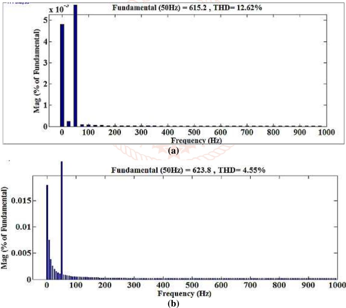
Figure 5.4 (a) THD at PCC without D-STATCOM and (b) THD at PCC with proposed control on D-STATCOM
