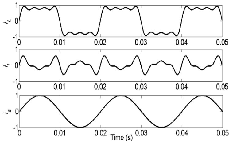
Fig 3.3 Current correction by DSTATCOM
