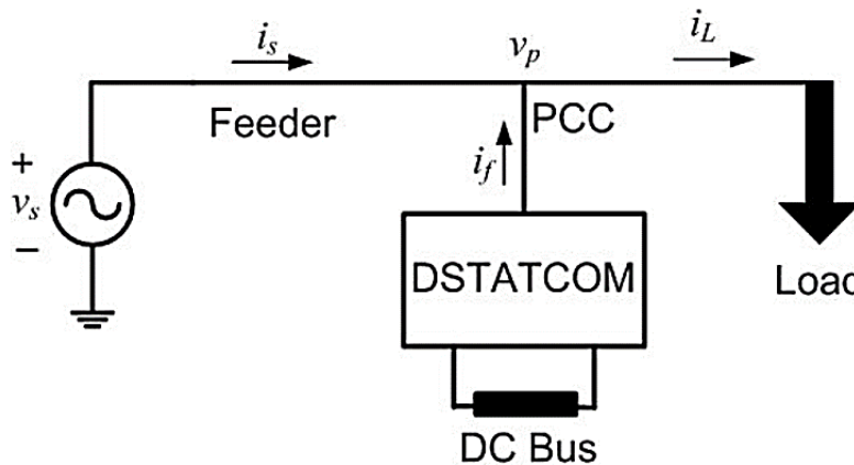
Fig. 1.3: Schematic diagram of DSTATCOM.
