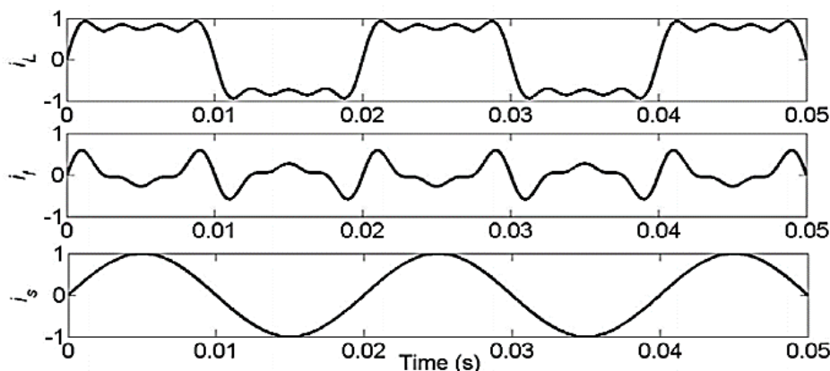
Fig. 1.4: Current correction by DSTATCOM.
