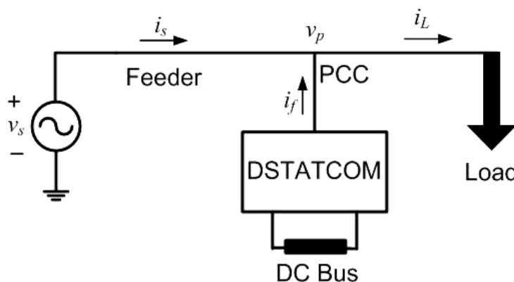
Fig. 3.2: Schematic diagram of DSTATCOM.
