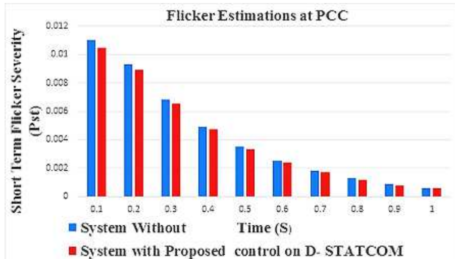
Fig 5.5: Flicker Estimations at PCC
