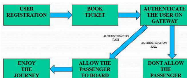
System Architecture
