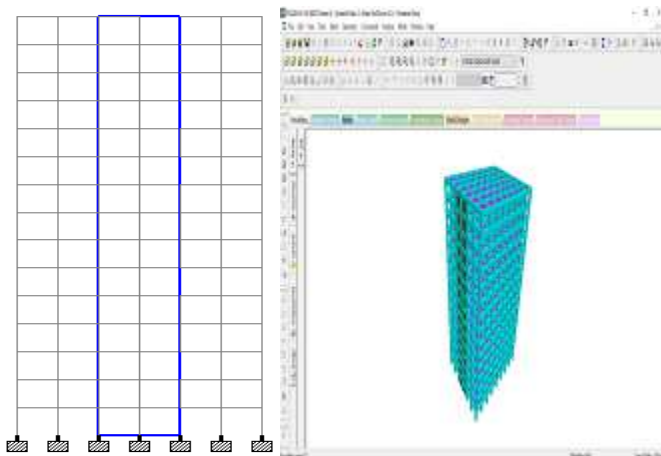
Figure 5 Framed building with Shear wall at the exterior side along X-direction. Zone- III & IV
