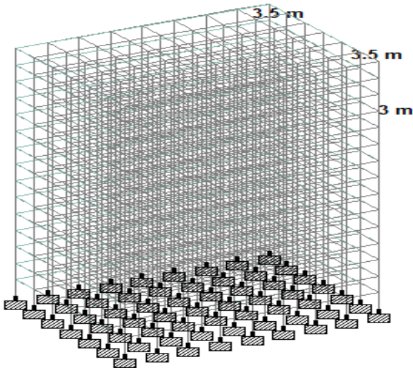
Figure 4 Model of the building
