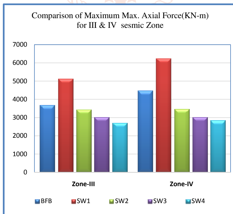
Figure 5.11: Comparison of Maximum. Axial Force
