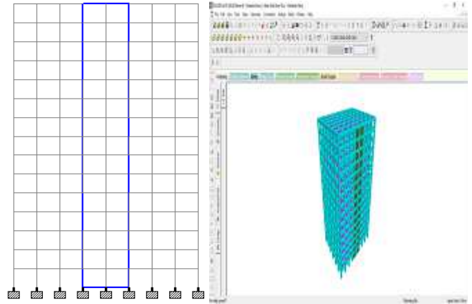
Figure 6 Framed building with Shear wall at the exterior side along Z-direction, Zone- III & IV
