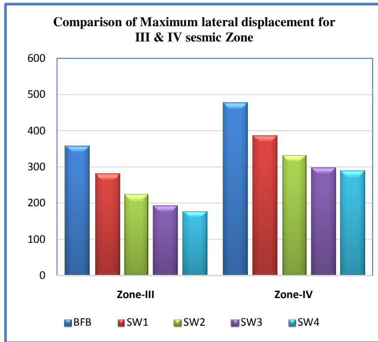
Figure 10: Comparison of Maximum lateral displacement
