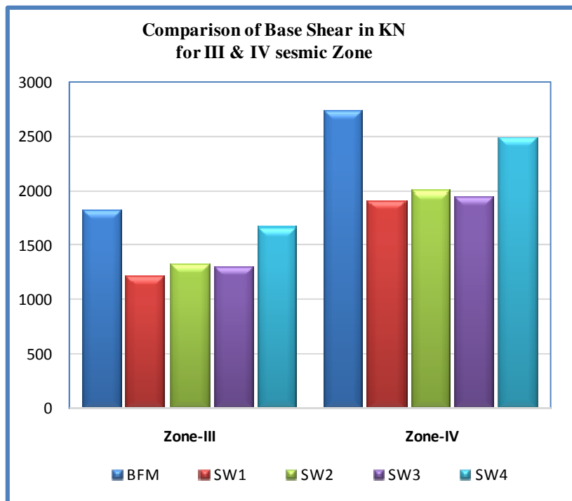
Figure-9: Comparison of Base Shear
