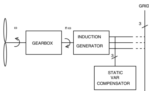
Fig 1 Wind turbine-based distributed generation scheme
