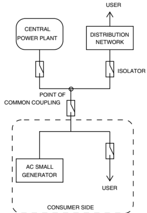
Fig 3 Demand side DG configurations with utility services
