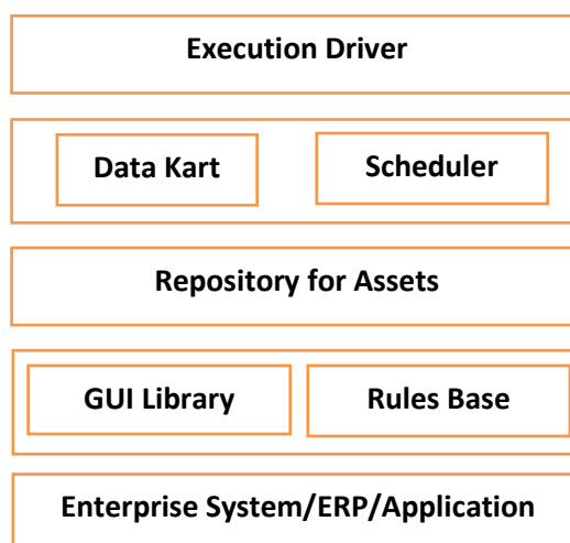
Figure 3: Advance Testing Architecture
