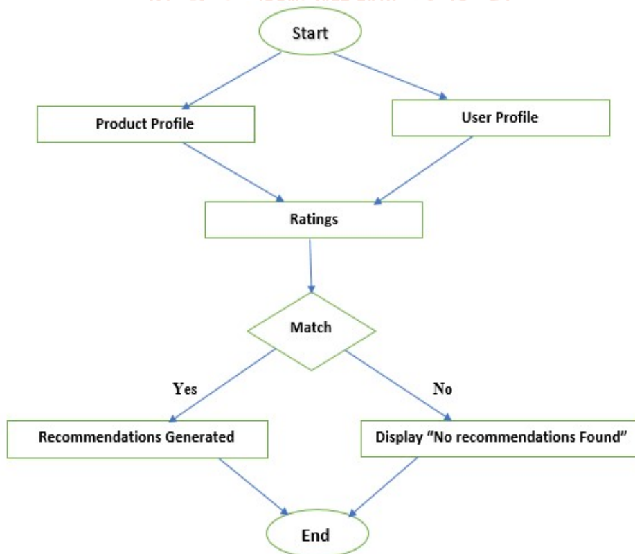
Figure.6 DFD diagram
