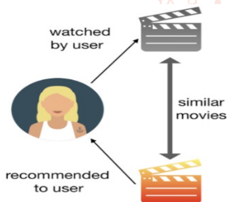
Figure1 Content-based filters
