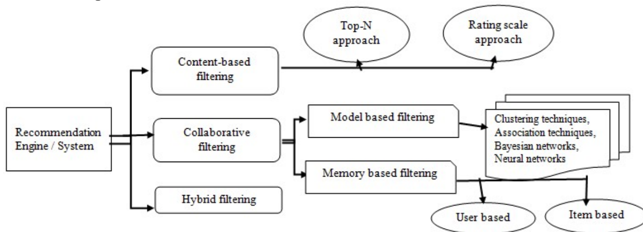
Figure.4: Architectural diagram
