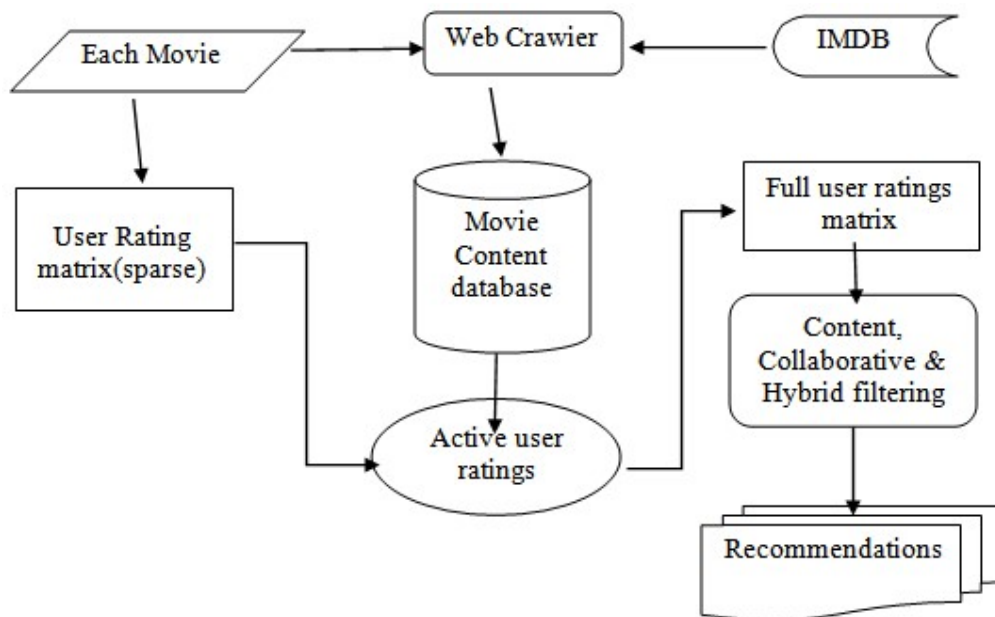
Figure.3 Hybrid method
