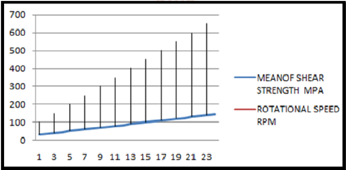
Fig 3.7: Variation of mean of shear strength at different rotational speeds
