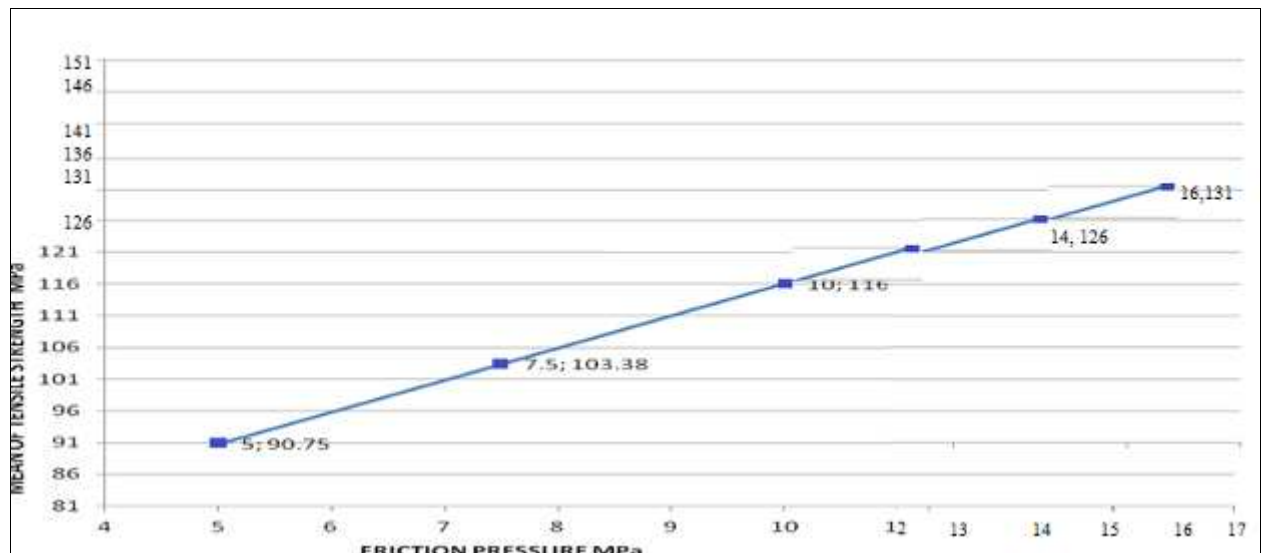
Fig 3.3: Variation of mean of tensile strength at different friction pressures
