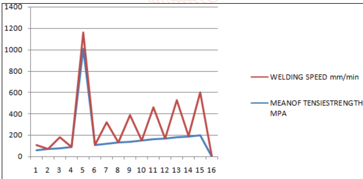
Fig 3.5: Variation of mean of tensile strength at different welding speeds
