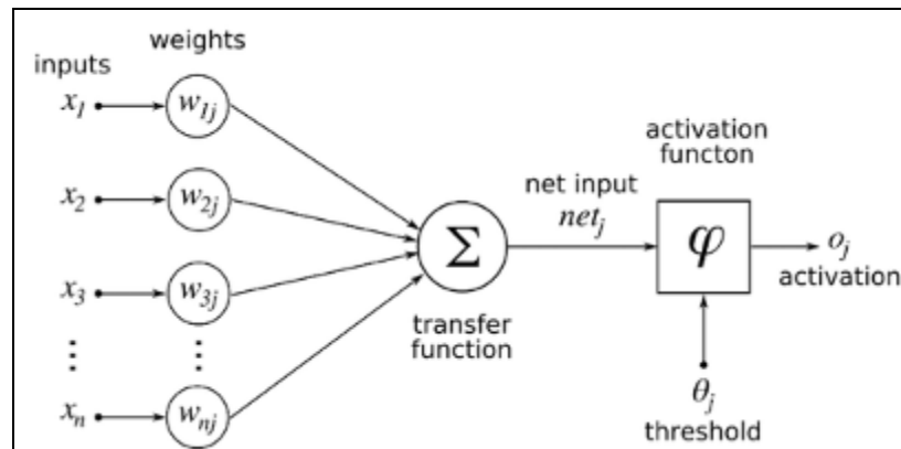
Fig1. Architecture of FFNN network model
