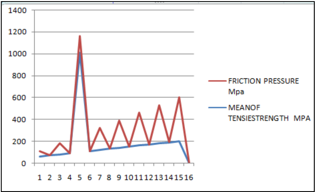
Fig 3.6: Variation of mean of shear strength at different friction pressures
