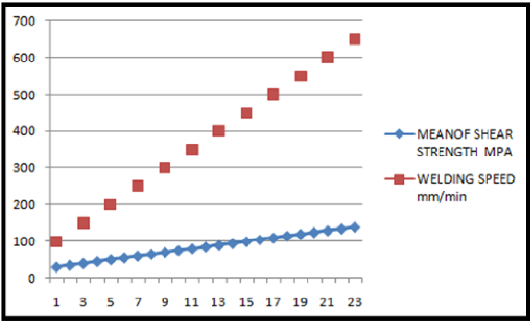
Fig 3.8: Variation of mean of shear strength with welding speeds
