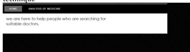
Fig1.Home Screen
