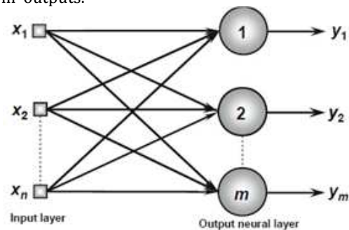
Figure 1 (Single-layer feed-forward network) ((da silva et al., 2017)
