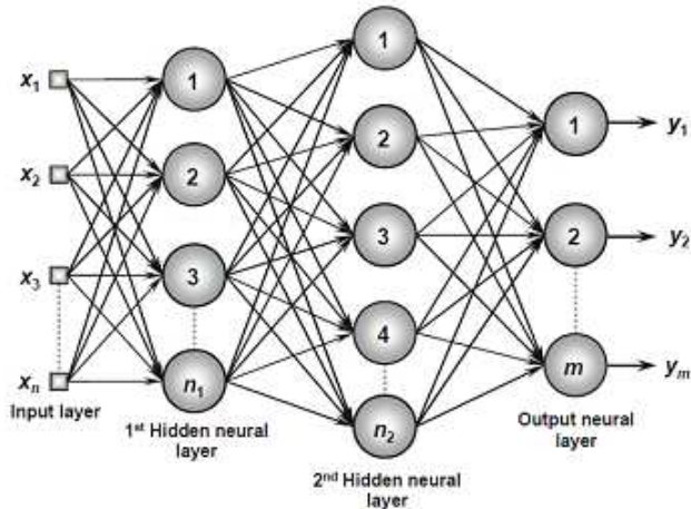
Figure 2 (Multiple-layer feed-forward network) (da silva et al., 2017)
