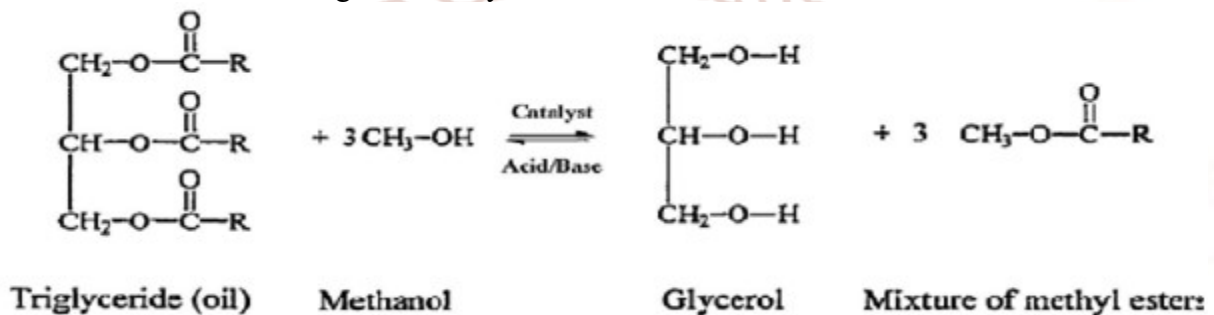
Fig 1: Transesterification reaction
