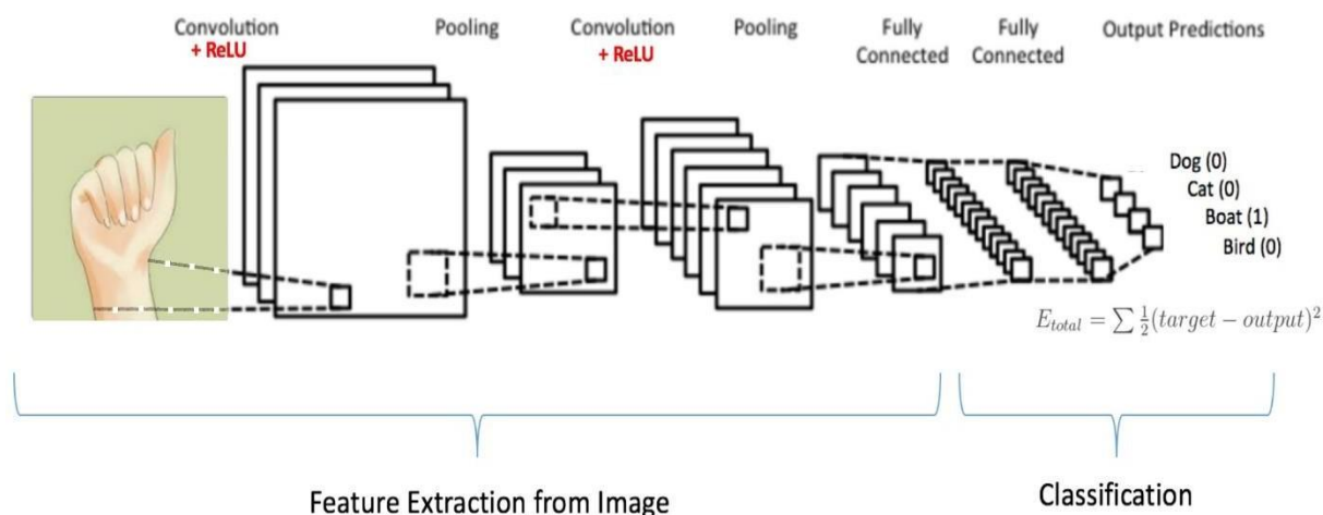
Figure 8:Convolutional Neural Network
