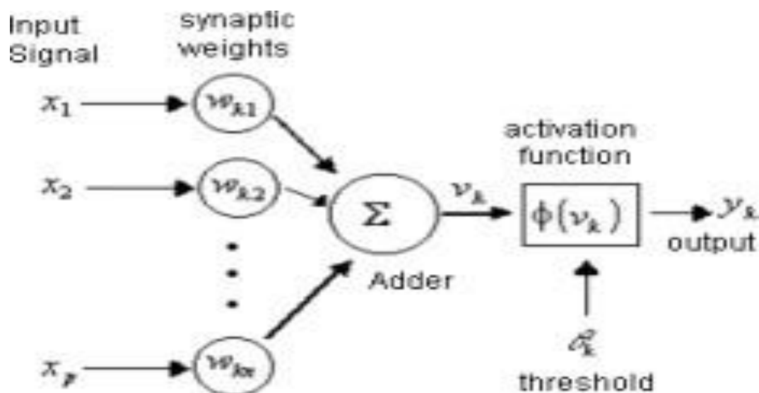
Figure 5 : Neural Network Model
