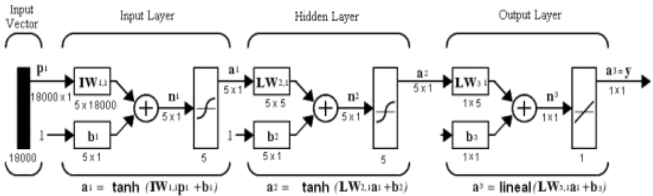
Figure 6: Employed Multilayer Neural Network
